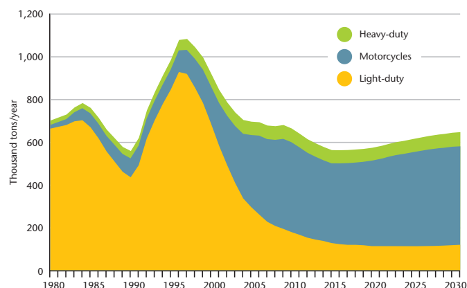
Figure 26: CO emissions in São Paulo (1980-2030)
