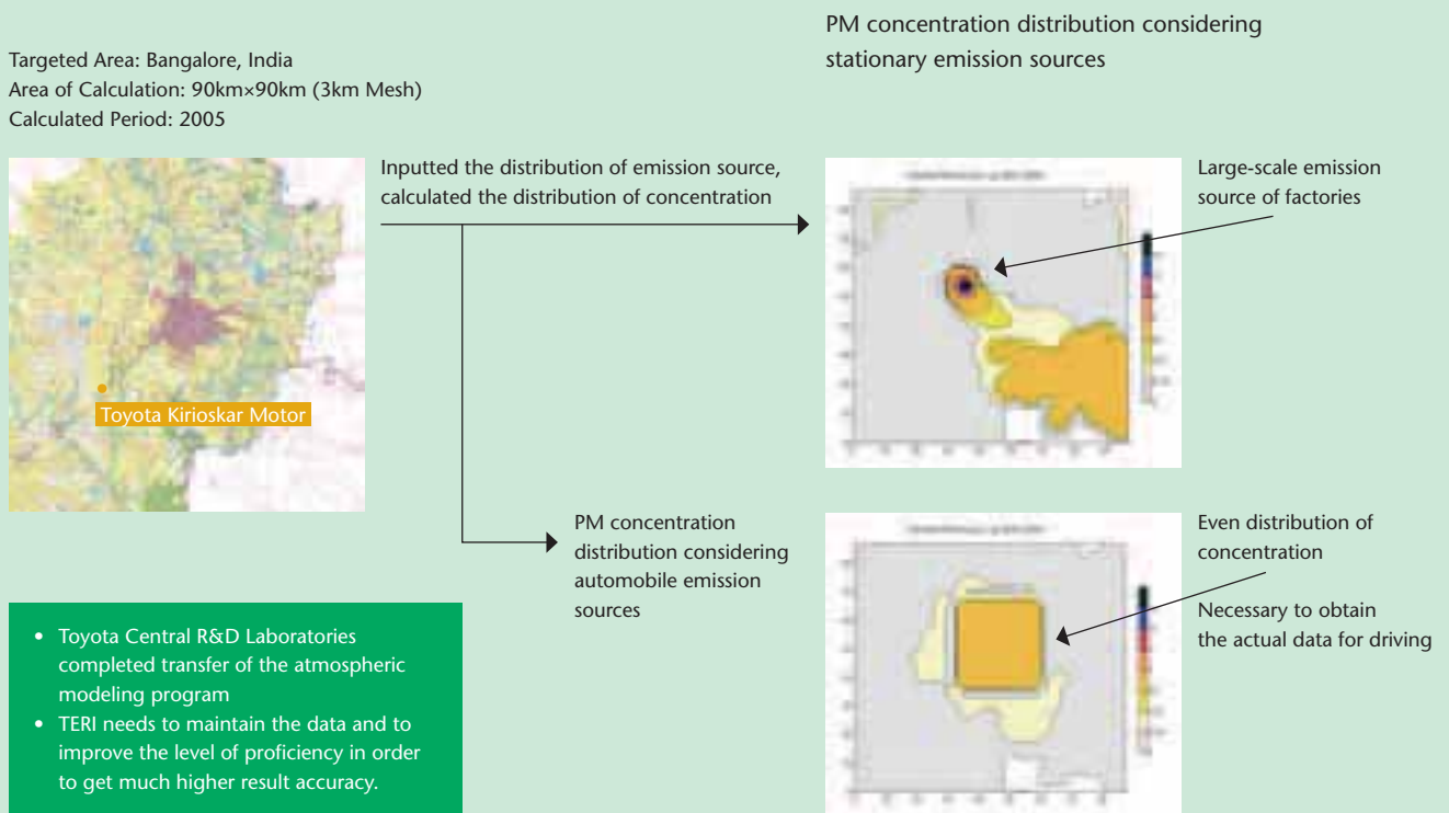
Figure 11: Results simulation of Bangalore atmospheric modeling
